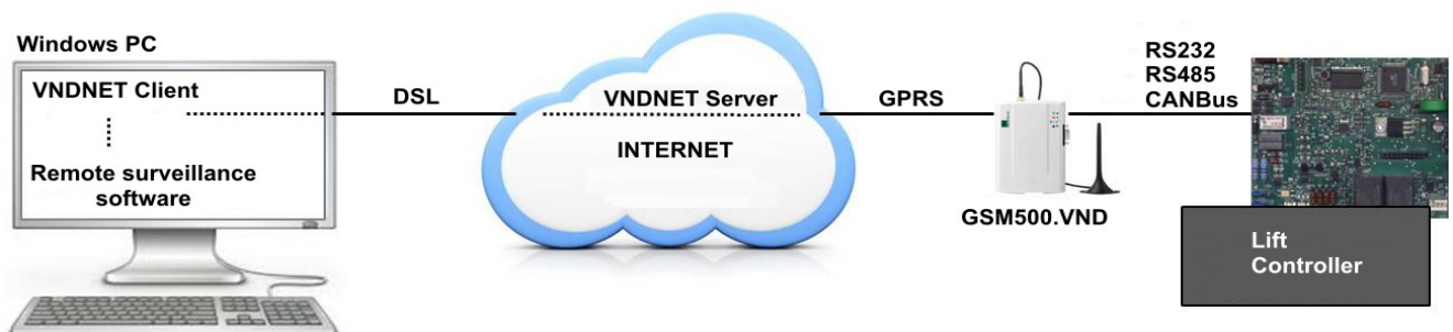
GSM500.3G Server supported data connectivity
