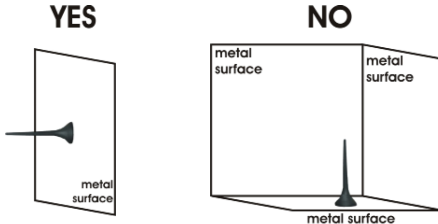
GSM500.3G Proper antenna positioning
